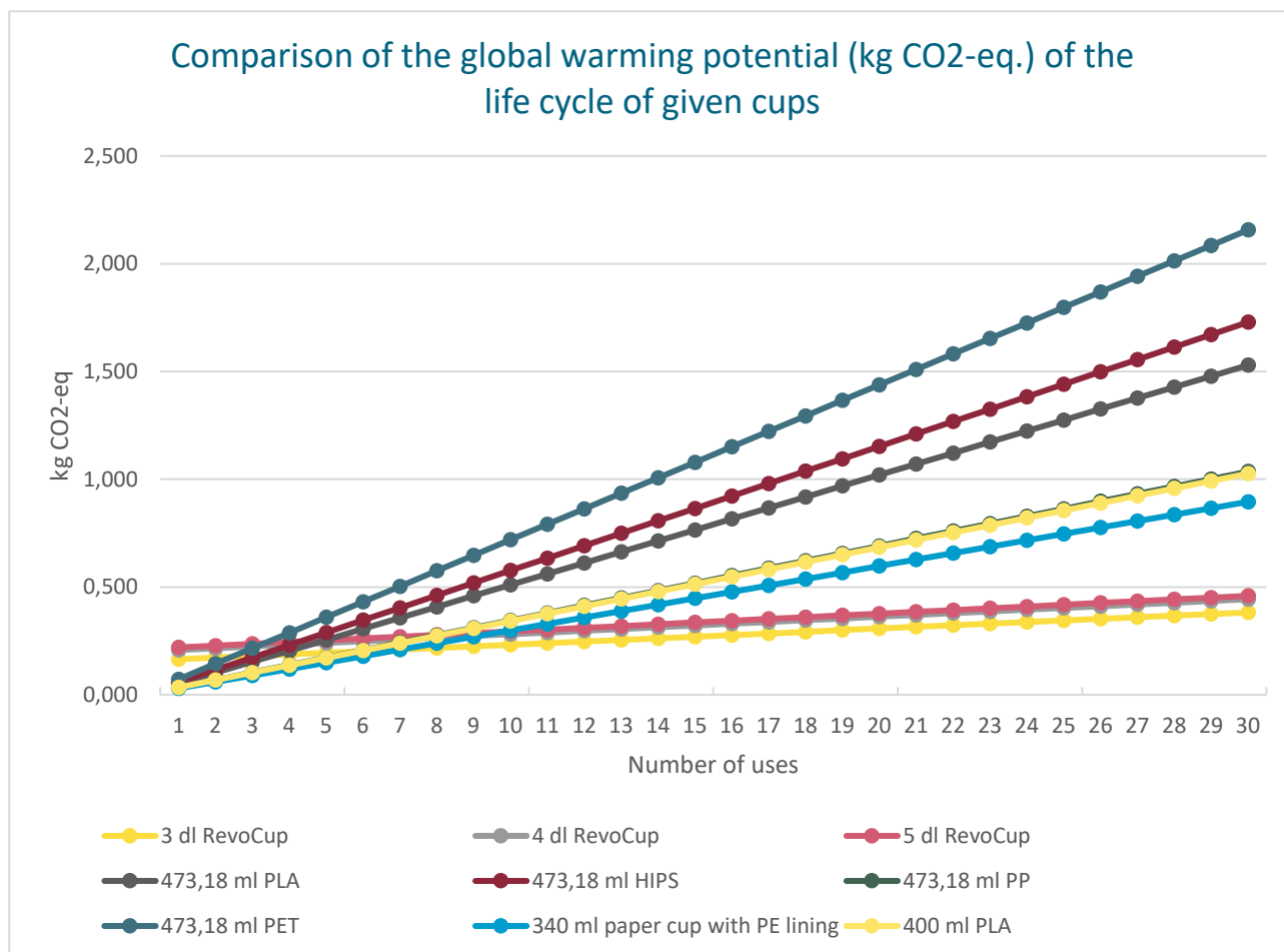
Figure 2 Comparison of RevoCup products with disposable cups
